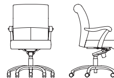
4862 Mid Back, Syncro-Tilt, Casters, Pneumatic Height Adjustment, Upholstered Arm Cap, Wood Sleeve W 27" D 25.75" H 41.5-44.5" SH 19.5-22.5" AH 27.5-30.5"
