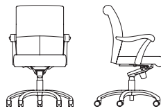
4762 Mid Back, Syncro-Tilt, Casters, Pneumatic Height Adjustment, Upholstered Arm Cap, Urethane Sleeve W 25.5" D 25" H 39-42" SH 18.5-21.5" AH 26.5-29.5"
