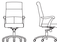
4775 High Back, Syncro-Tilt, Casters, Pneumatic Height Adjustment, Urethane Arm Cap, Urethane Sleeve W 25.5" D 23" H 45-48" SH 18.5-21.5" AH 26.5-29.5"
