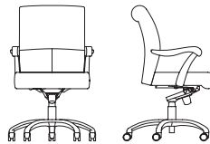
4865 Mid Back, Syncro-Tilt, Casters, Pneumatic Height Adjustment, Urethane Arm Cap, Wood Sleeve W 27" D 25.75" H 41.5-44.5" SH 19-22" AH 27.5-30.5"
