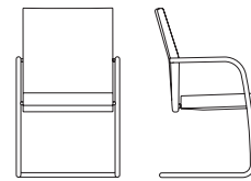
7102 Mid Back, Sled Base W 22.5" D 22.5" H 37" SH 18.5" AH 26.5"
