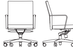
7211 Mid Back Tilter, Aluminum Arm & Base W 27" D 27" H 35.5-39.25" SH 16.75-20.5" AH 24.5-28.5"
