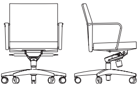
7201 Low Back Tilter, Aluminum Arm & Base W 27" D 27" H 32.5-36.25" SH 16.75-20.5" AH 24.5-28.25"
